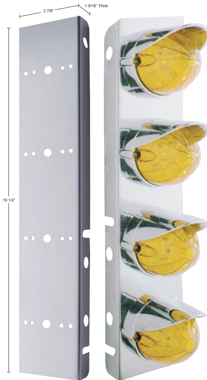
Stainless Steel Bracket Only Item # 30975-1
